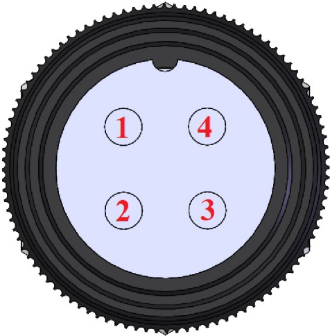
Vista Frontal Conector ITC Fêmea
